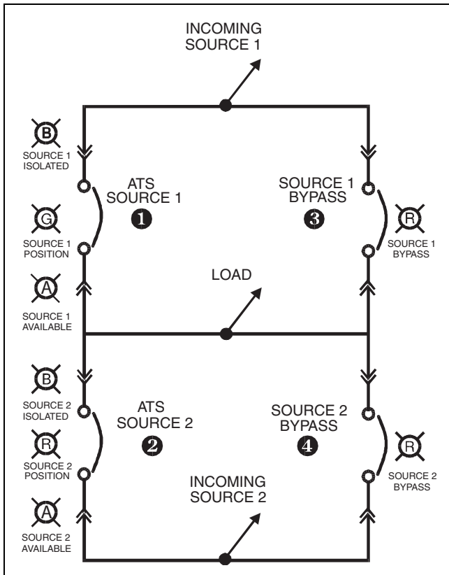
Figure 4. Typical Bypass Isolation Switch Schematic.
