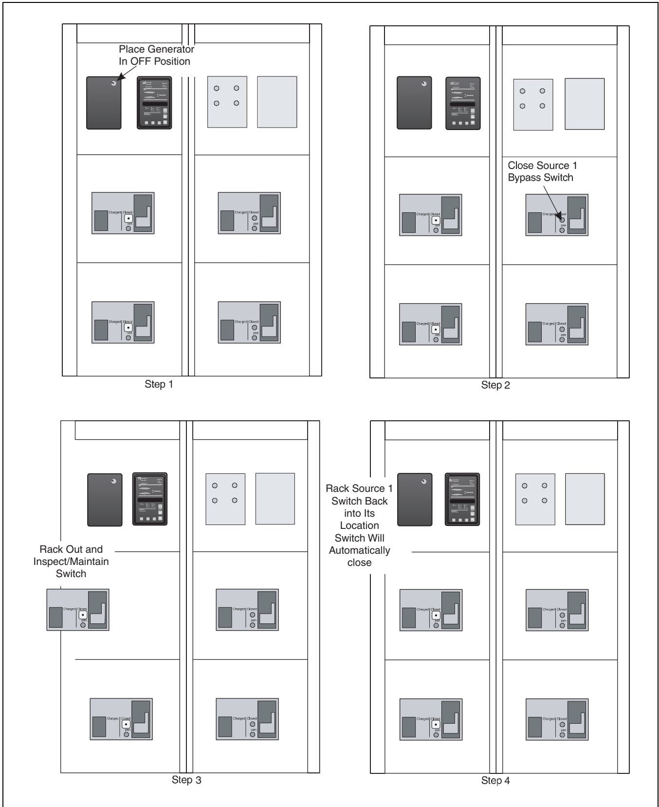
Figure 37. Transfer from Normal Switching Device to Normal Bypass Switching Device, Steps 1-4.
