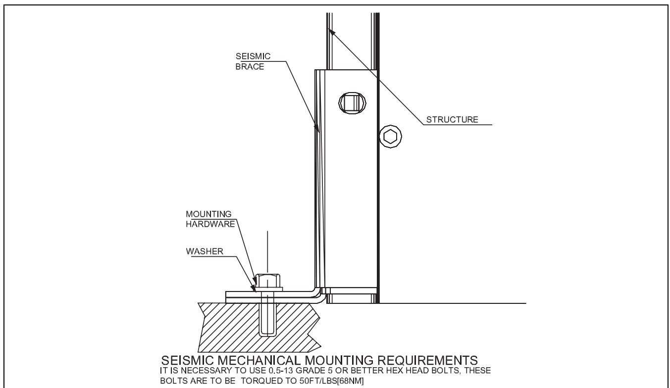
Figure 20. Seismic Tested and Approved Product Mounting Instructions.
