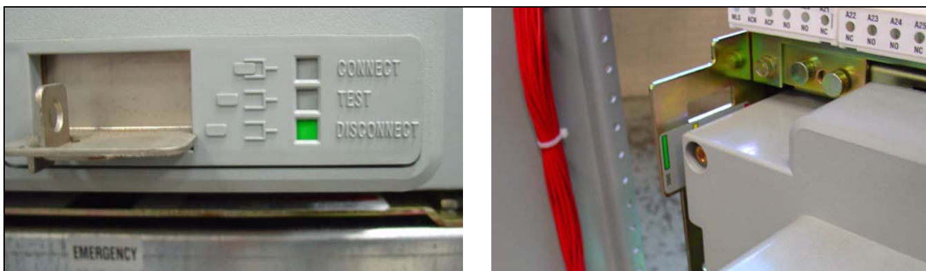
Figure 31. Switching Device in the DISCONNECT Position.
