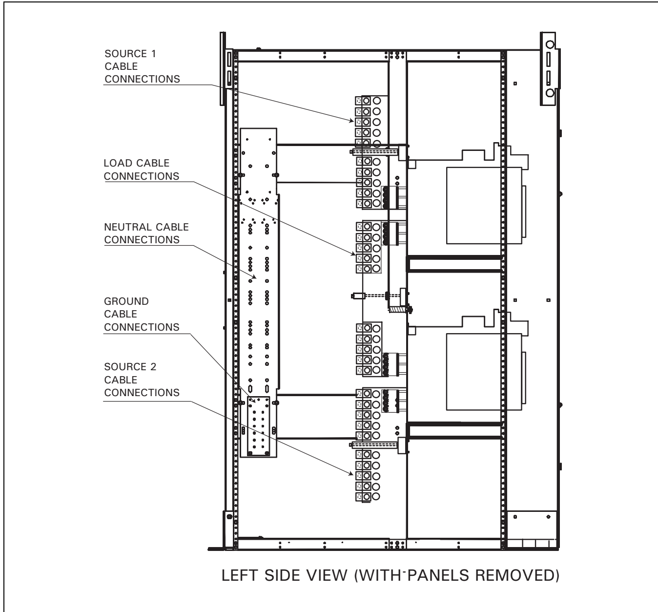
Figure 13. Terminal Connections for a Typical Drawout Transfer Switch (800-3200A Closed Transition Shown).
