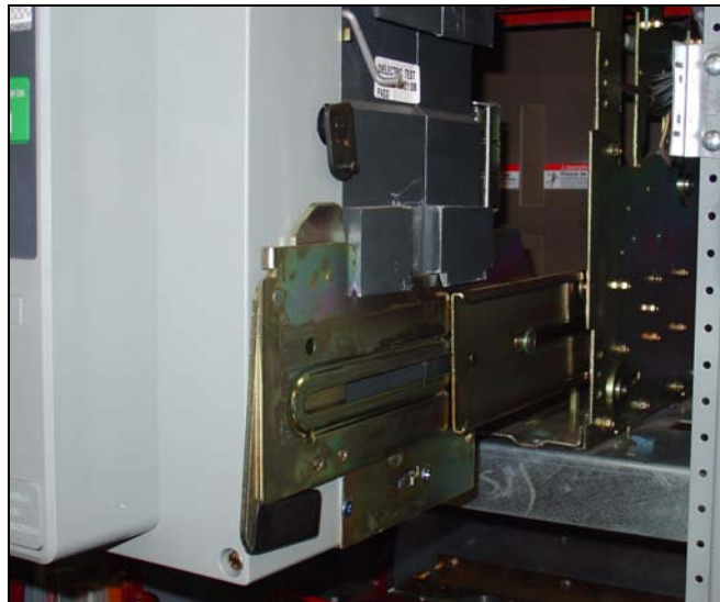
Figure 22. One Side of Drawout Circuit Breaker Properly Seated on Extension Rails.
