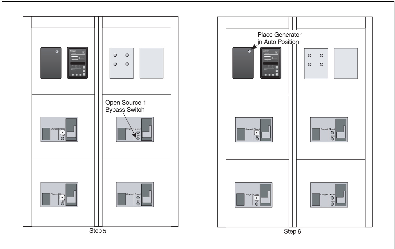
Figure 38. Transfer from Normal Switching Device to Normal Bypass Switching Device, Steps 5-6
