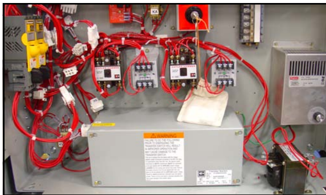
Figure 15. Voltage Selection Panel
