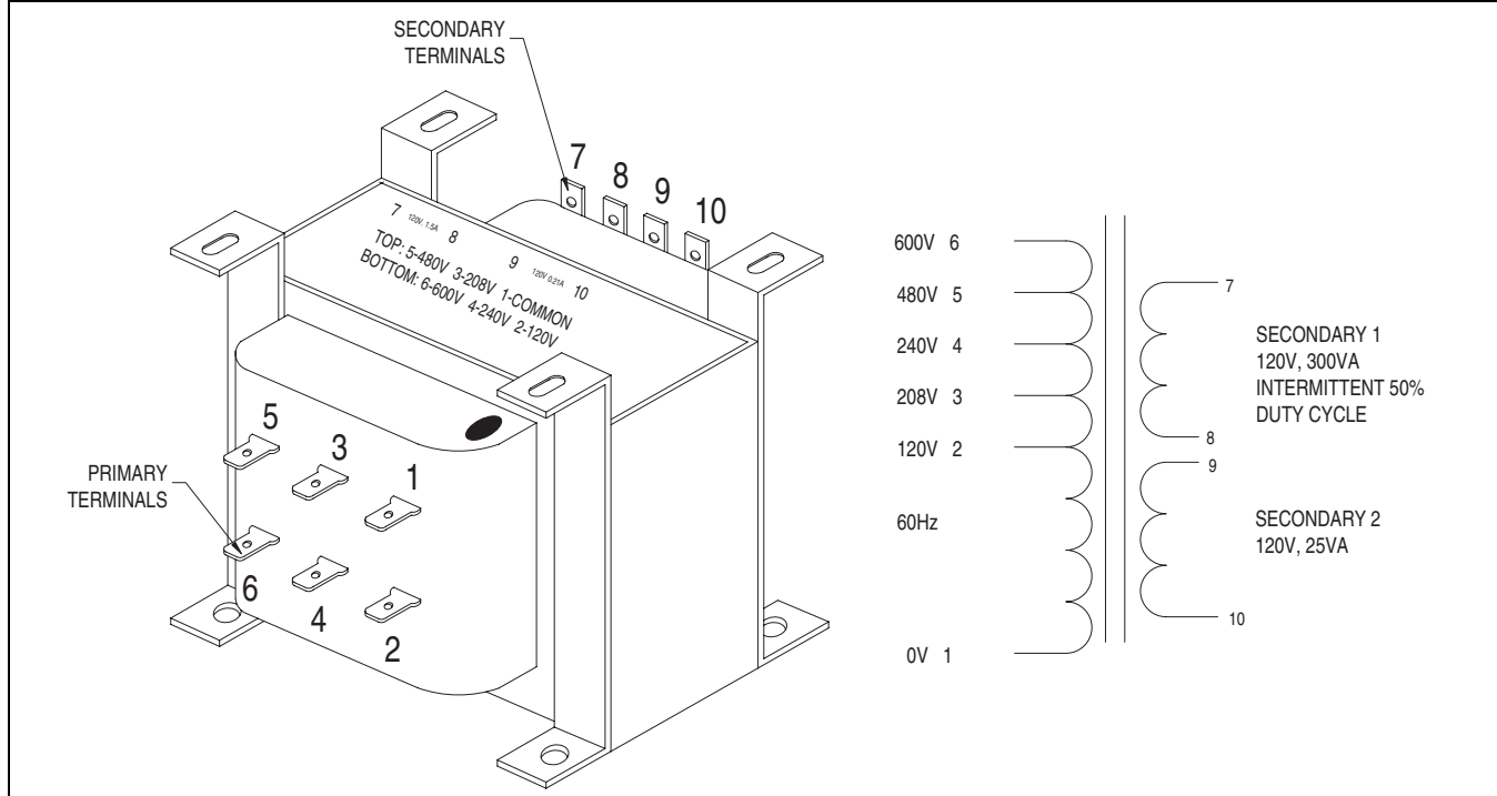
Figure 21. Voltage Selection Adjustment
