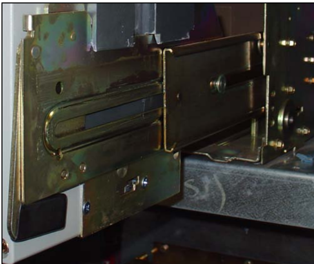
Figure 27. Drawout Rail Supports Fully Seated in the Rail Cutouts.
