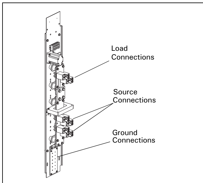
Figure 18. Neutral SE with Ground Fault
