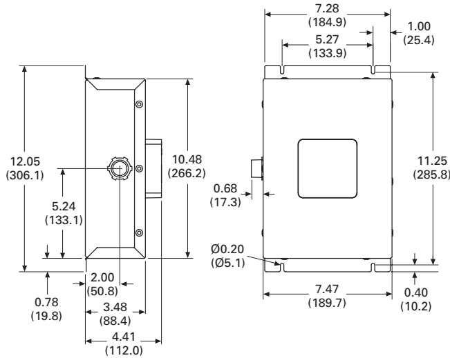
250–400 kA Units in a NEMA 1 Rated Enclosure, Weight = 13.5 lbs
